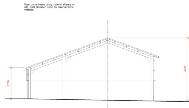
East Elevation 1:100
